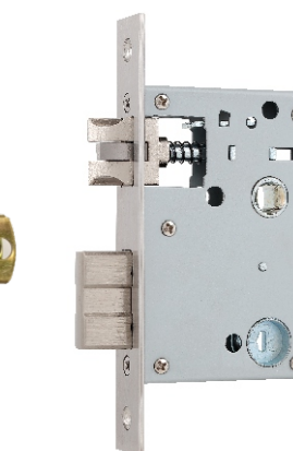
Lockcase(50/50mm)
